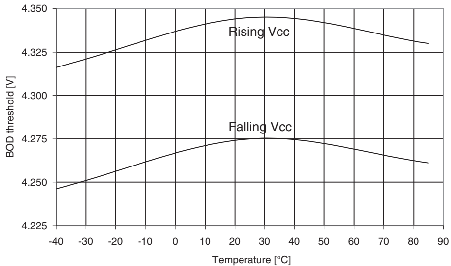
Figure 31-224. ATmega329PA: BOD Thresholds vs. temperature (BOD level is 4.3V).
