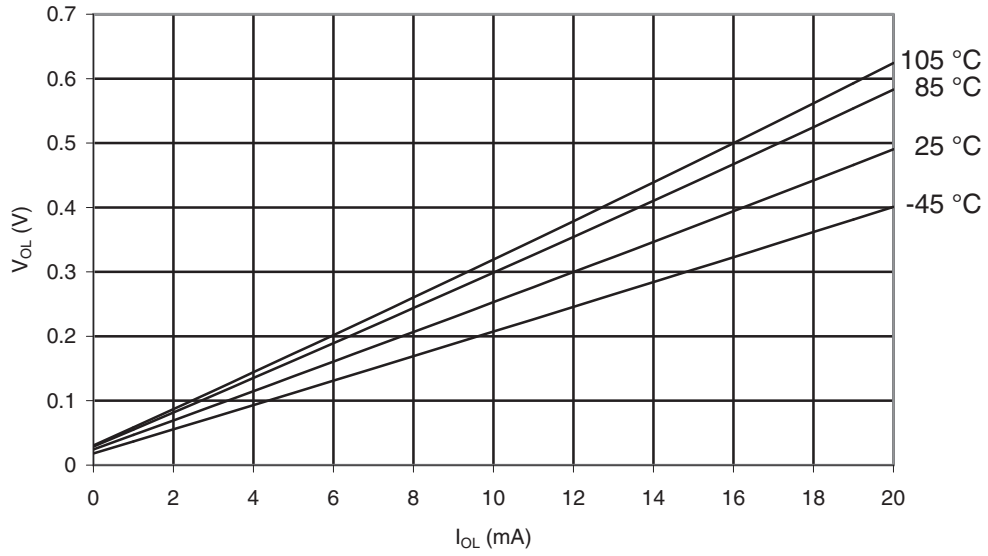
Figure 32-30. ATmega169PA-105°C: I/O Pin Output Voltage vs. Sink Current, PortB ( V_{CC}= 5V )
