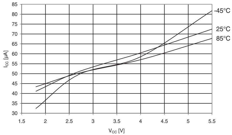
Figure 31-58. ATmega169A: Analog Comparator current vs. V_{CC} .
