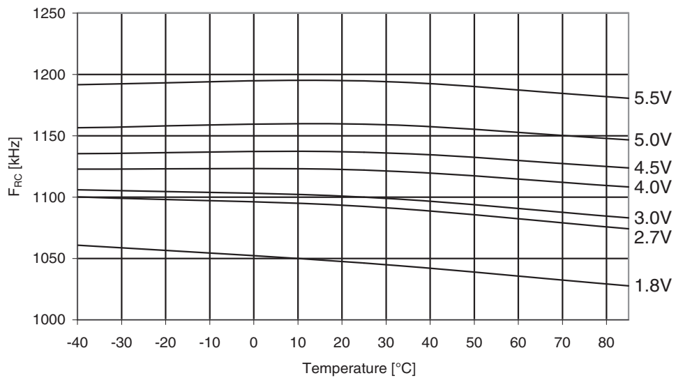
Figure 31-290. ATmega3290A: Watchdog Oscillator frequency vs. temperature.
